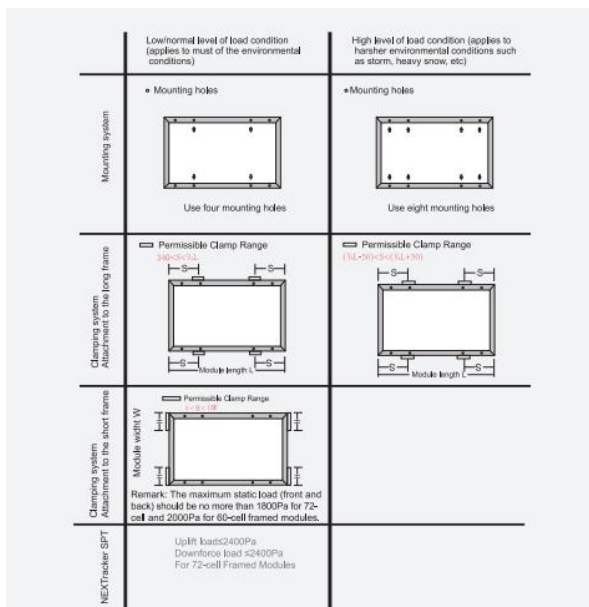
Figure 4 Installation Methods
